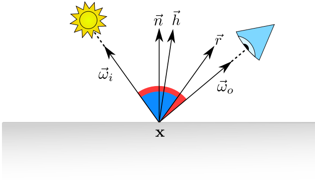
Figure 3.6: Glossy vectors for microfacet theory. The blue angles are the same for the reflection vector, the red ones are the same for the half vector.
