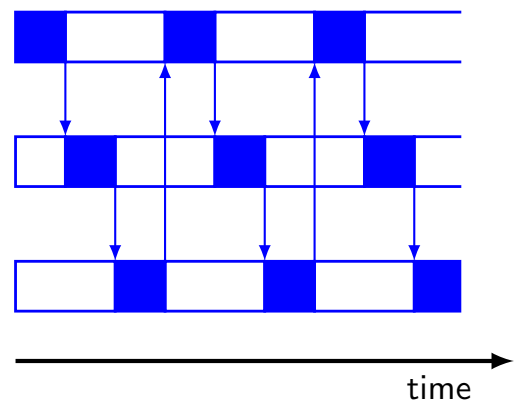
User-space threads
