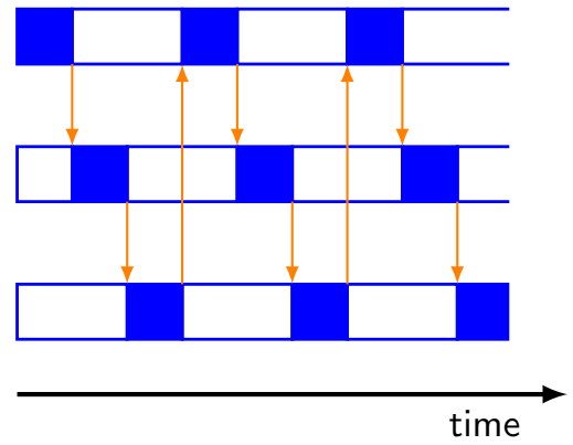
Multi-tasking
