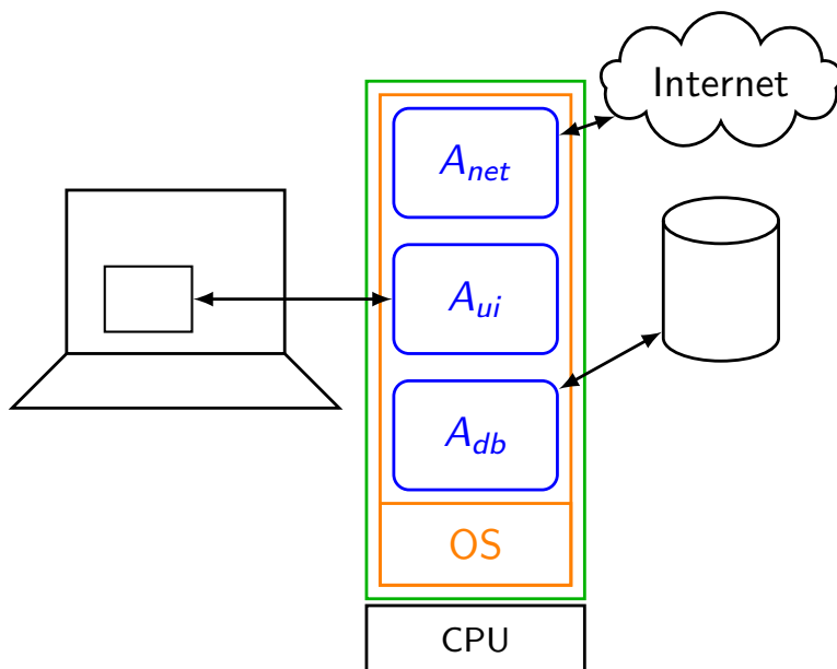
User-space threads
