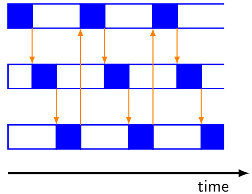
Time-sharing
