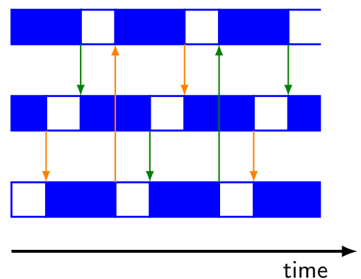
Multi-processing
