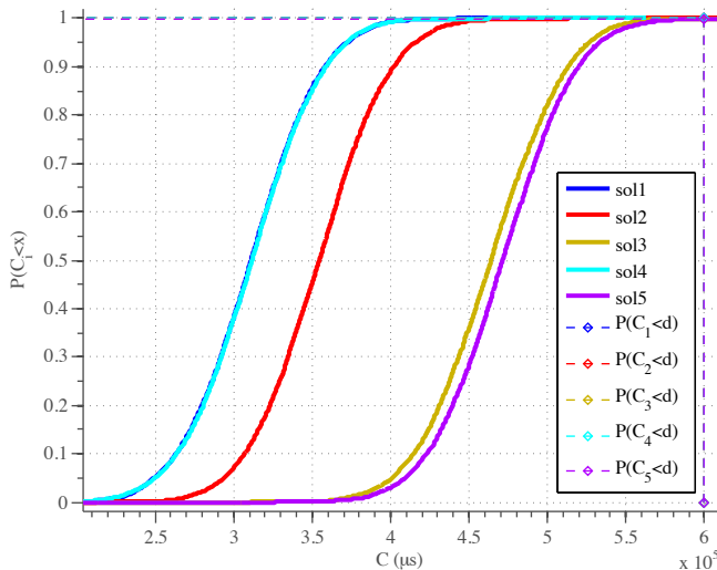
Figure 4.6: Comparison of the CDF of different clustering solutions for MJPEG encoder
