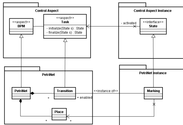
Fig. 10. A Petri net implementation
