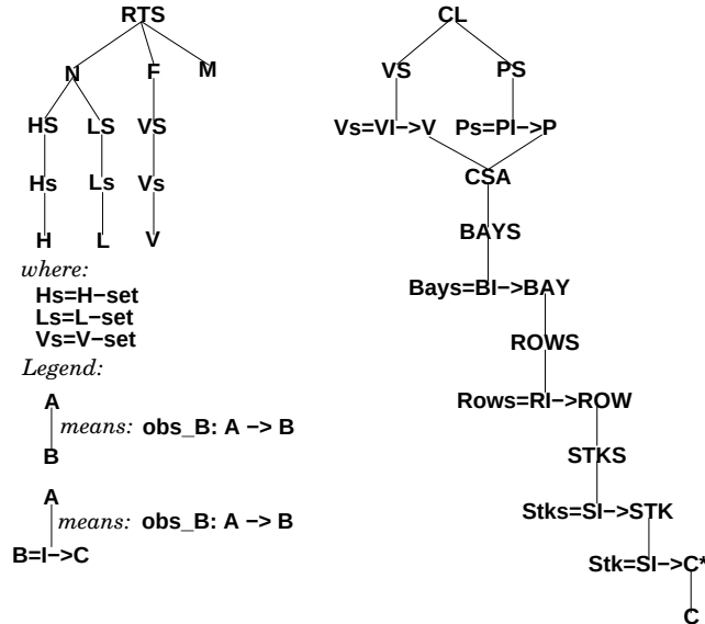
Figure 1: Two Domain Lattices: Examples 9 on page 10 and 11 on the preceding page
